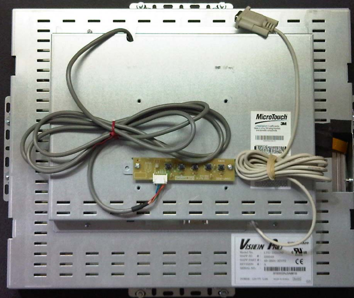
49-2765-19G3 LCD Metal Mounting Bracket Installation Note: Mounting is done on all four sides to improve the stability of mounting. This fixes old problem when one pushed on top and bottom of lcd it moved away from front of bracket.
